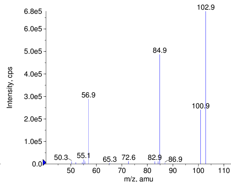
■ - gamma-Hydroxybutyric acid Prec(103.0) CE(-99.0) RT(0.9)
