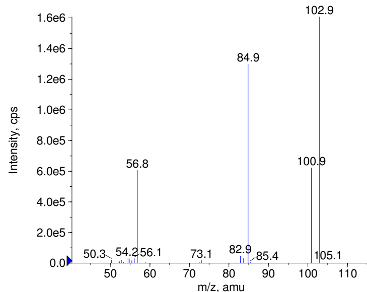
■ - gamma-Hydroxybutyric acid Prec(103.0) CE(-50.0) RT(0.9)
