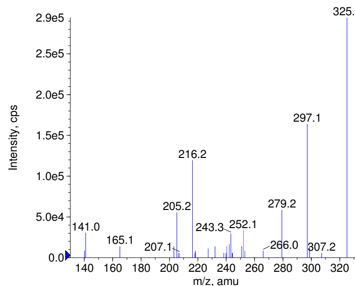
+ alpha-Hydroxyalprazolam Prec(325.0) CE(99.0) RT(0.7)
