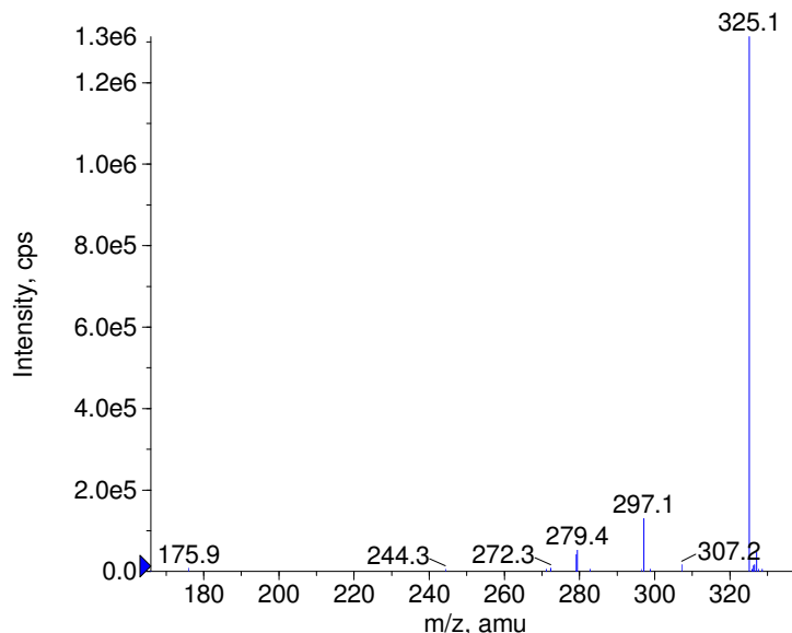
+ alpha-Hydroxyalprazolam Prec(325.0) CE(50.0) RT(0.7)
