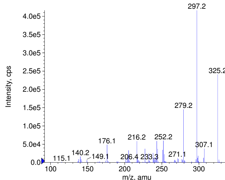
+ alpha-Hydroxyalprazolam Prec(325.0) CE(99.0) RT(0.7)
