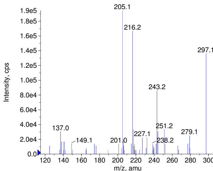
+ alpha-Hydroxyalprazolam Prec(325.0) CE(50.0) RT(0.7)
