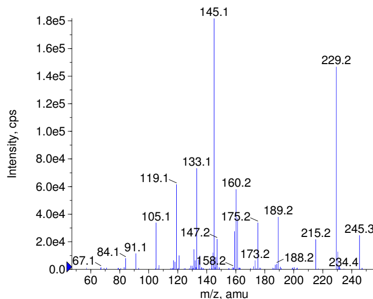
+ Xylometazoline Prec(245.0) CE(50.0) RT(0.9)
