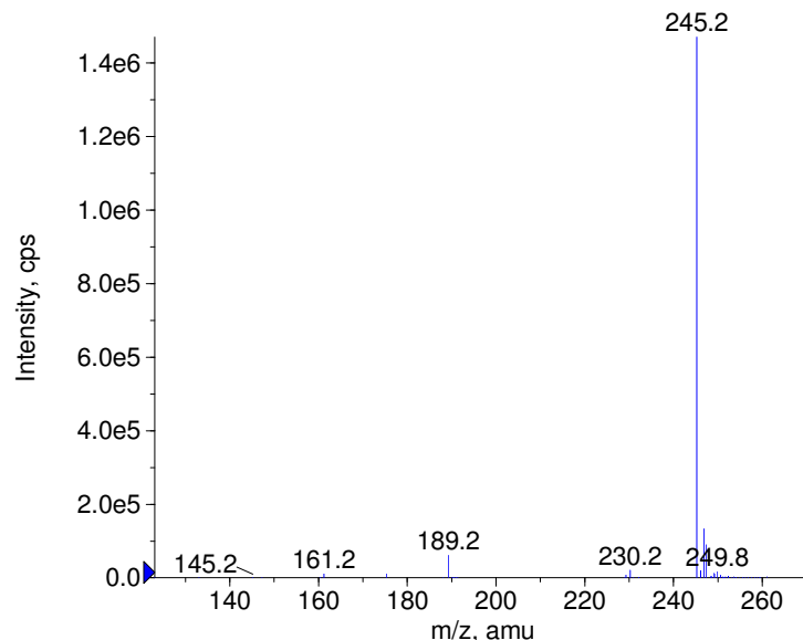
+ Xylometazoline Prec(245.0) CE(50.0) RT(0.9)
