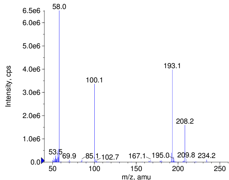
+ Trimipramine Prec(295.0) CE(50.0) RT(0.8)
