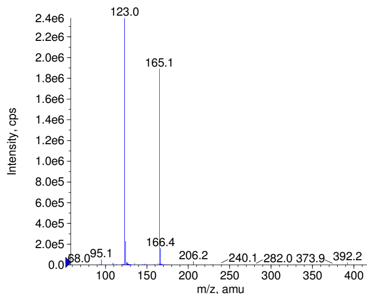
■ + Trifluoperidol Prec(410.0) CE(50.0) RT(0.8)
