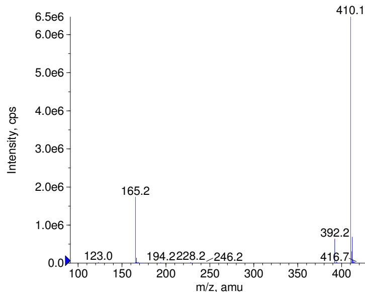
■ + Trifluoperidol Prec(410.0) CE(50.0) RT(0.8)
