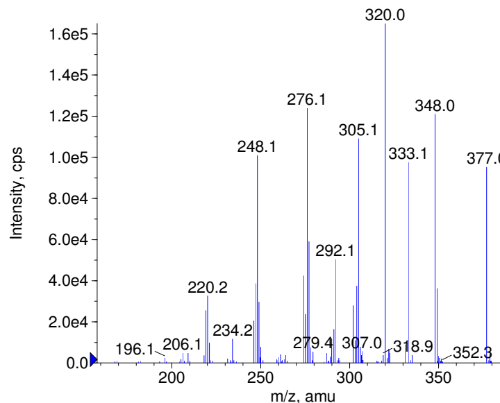
■ + Topotecan Prec(422.0) CE(50.0) RT(0.9)
