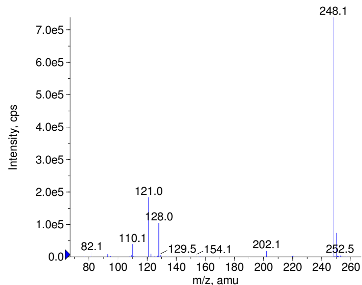
+ Tinidazole Prec(248.0) CE(50.0) RT(0.9)
