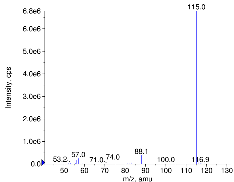
+ Thiamazole Prec(115.0) CE(50.0) RT(1.0)
