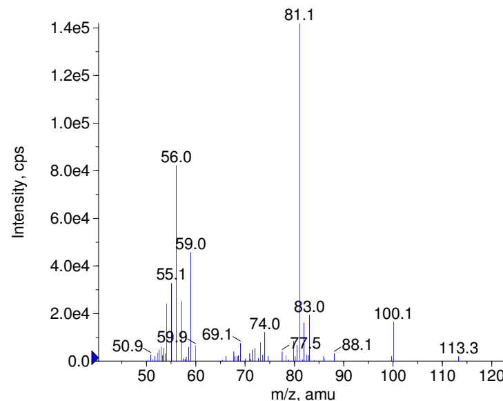
+ Thiamazole Prec(115.0) CE(50.0) RT(1.0)
