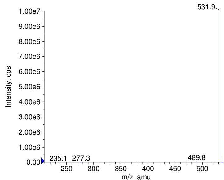
+ Terconazole Prec(532.0) CE(50.0) RT(0.7)
