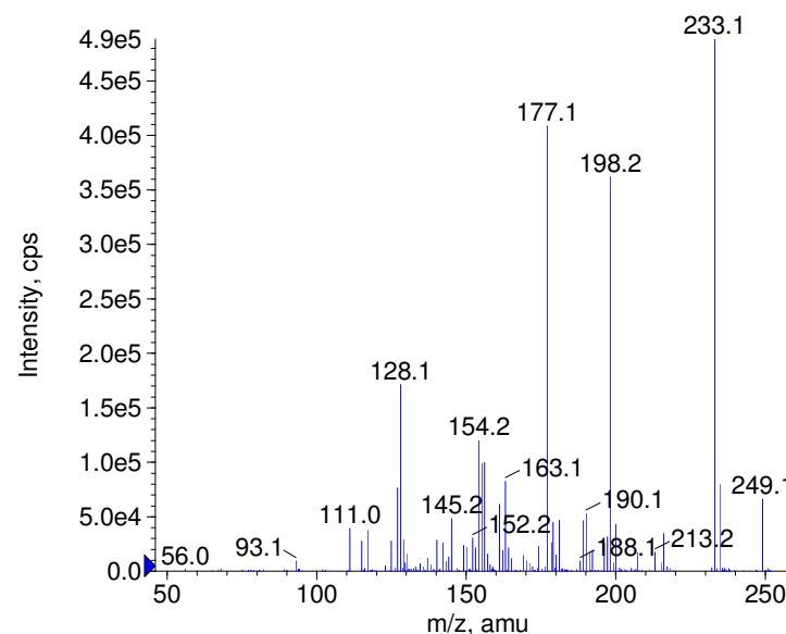
+ Pyrimethamine Prec(249.0) CE(50.0) RT(0.9)
