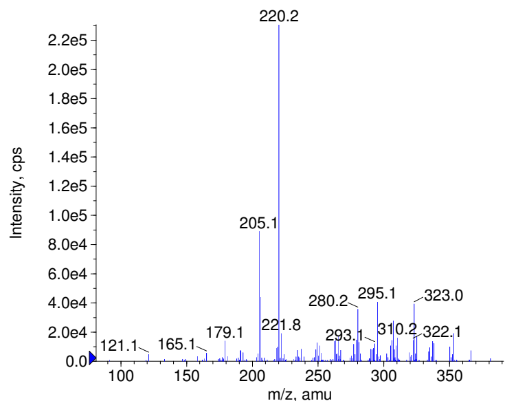
■ + Noscapine Prec(414.0) CE(50.0) RT(0.7)
