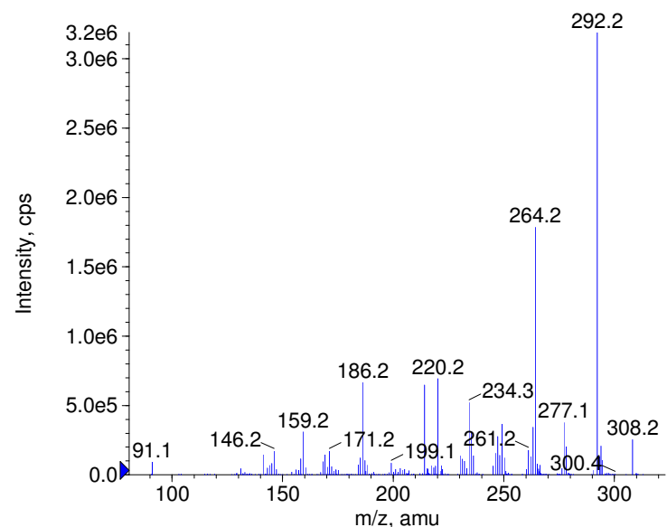
+ Moxaverine Prec(308.0) CE(50.0) RT(0.8)
