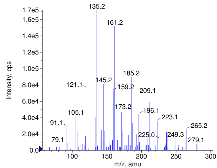
■ + Methylprednisolone Prec(375.0) CE(50.0) RT(1.3)
