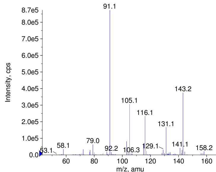
+ Isoaminile Prec(245.0) CE(50.0) RT(0.9)
