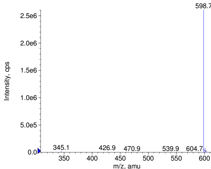
■ + Iopodic acid Prec(599.0) CE(50.0) RT(1.2)
