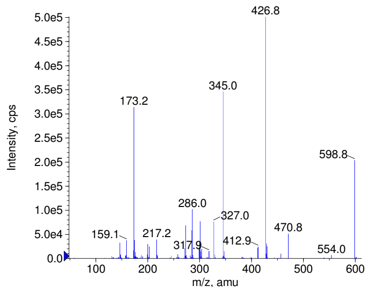
■ + Iopodic acid Prec(599.0) CE(50.0) RT(1.2)
