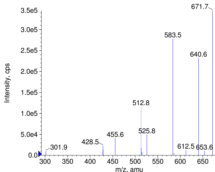
+ Ioglicic acid Prec(672.0) CE(50.0) RT(0.9)
