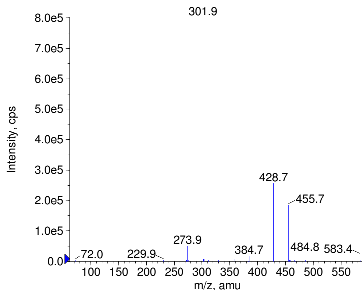
+ Ioglicic acid Prec(672.0) CE(50.0) RT(0.9)
