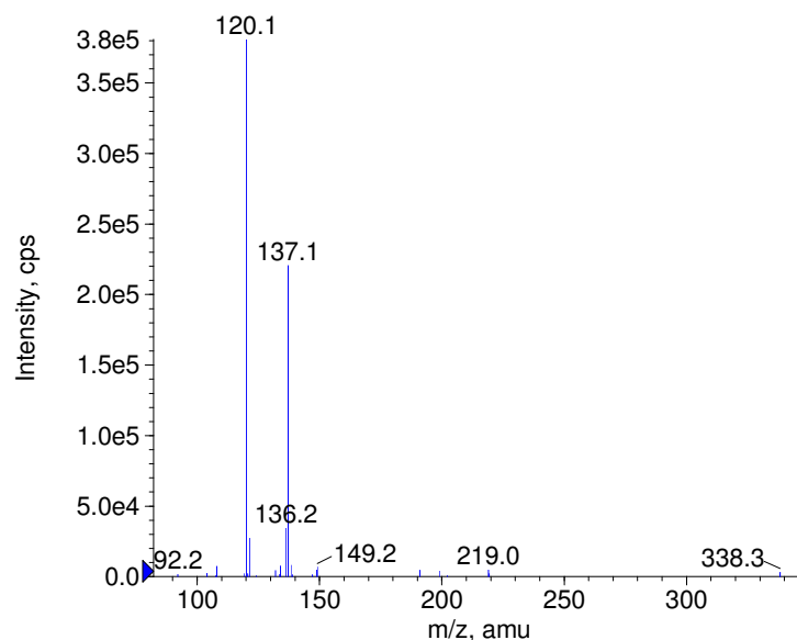
■ + Hexamidine Prec(355.0) CE(50.0) RT(0.8)
