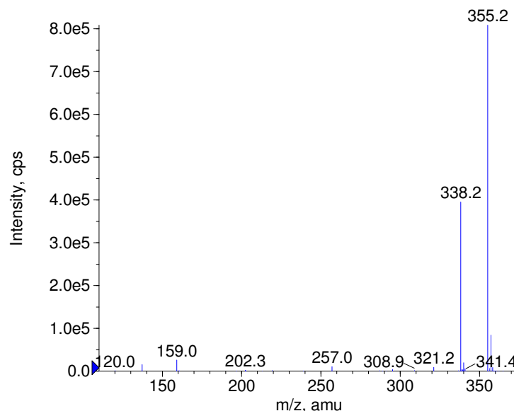
■ + Hexamidine Prec(355.0) CE(50.0) RT(0.8)
