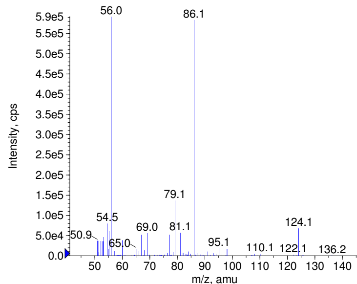
+ Guanacine Prec(183.0) CE(50.0) RT(1.6)
