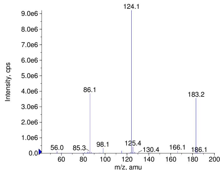
+ Guanacine Prec(183.0) CE(50.0) RT(1.6)
