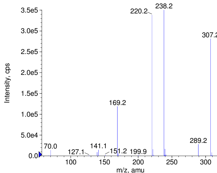
+ Fluconazole Prec(307.0) CE(50.0) RT(0.7)
