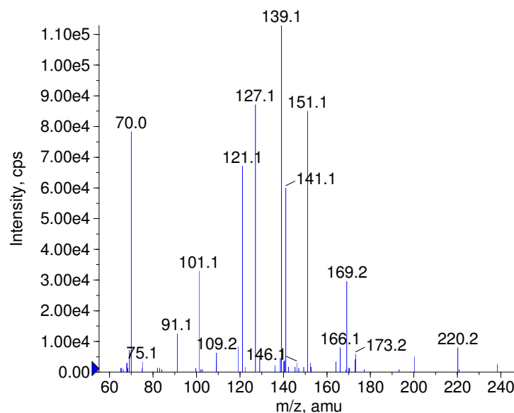
+ Fluconazole Prec(307.0) CE(50.0) RT(0.7)
