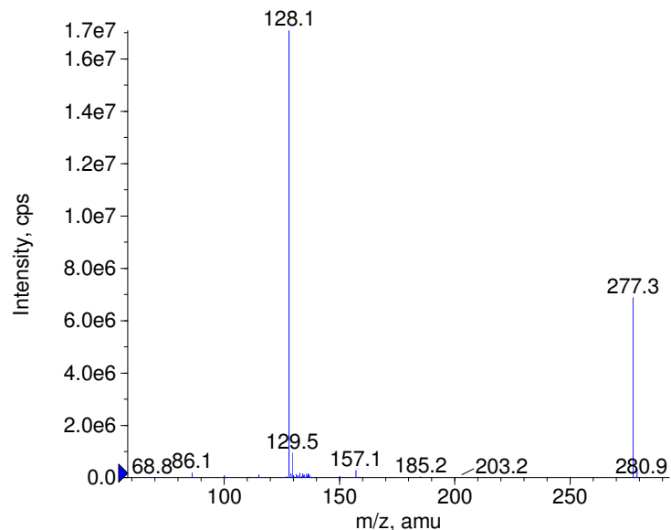
+ Etidocaine Prec(277.0) CE(50.0) RT(0.8)
