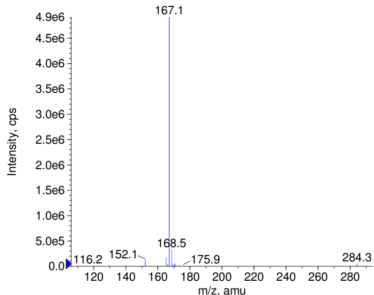
+ Ethylbenzhydramine Prec(284.0) CE(50.0) RT(0.9)
