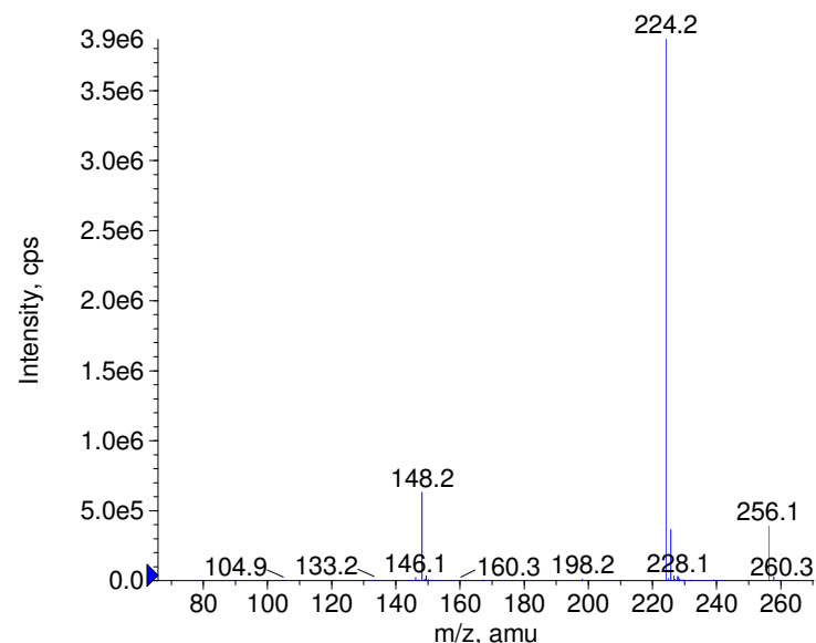
+ Dimethachlor Prec(256.0) CE(50.0) RT(1.1)
