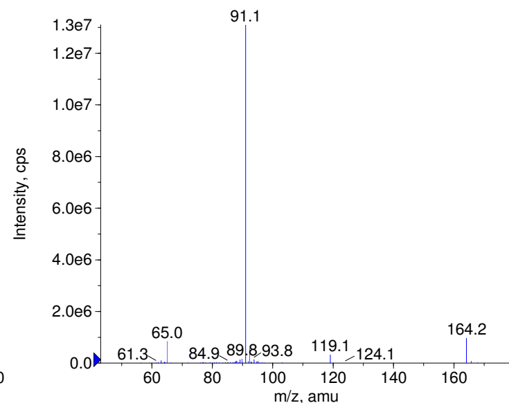
+ Dimephenopam Prec(164.0) CE(99.0) RT(0.9)
