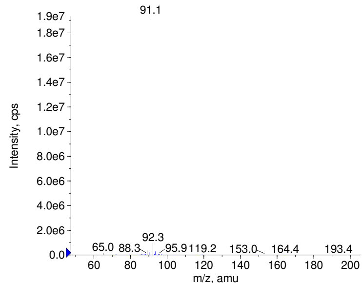
+ Dimephenopam Prec(164.0) CE(99.0) RT(0.9)
