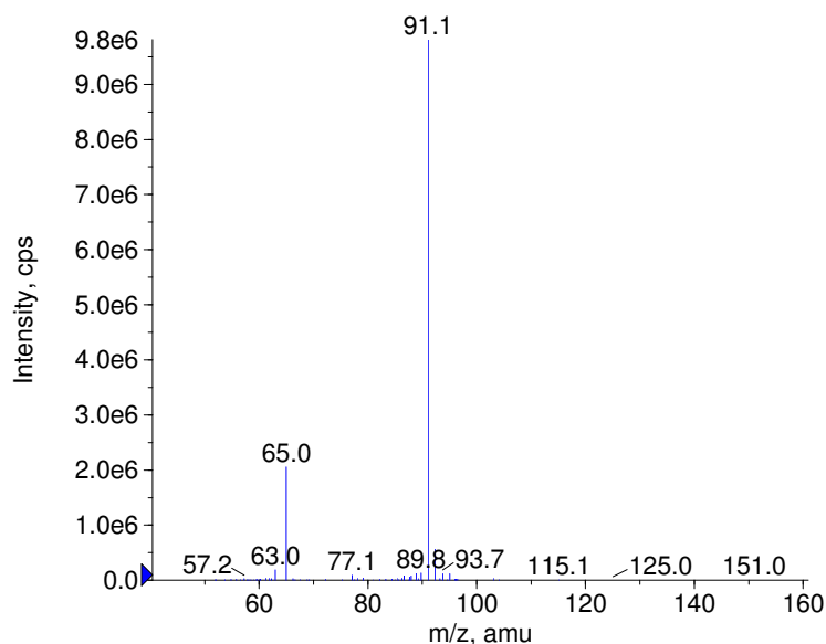
+ Dimephenopam Prec(164.0) CE(50.0) RT(0.9)
