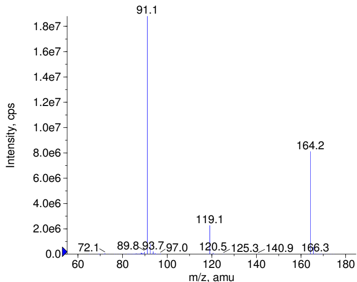
+ Dimephenopam Prec(164.0) CE(50.0) RT(0.9)
