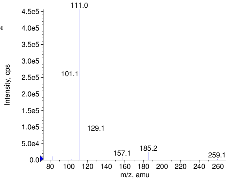
+ Dibutyl adipate Prec(259.0) CE(50.0) RT(3.7)
