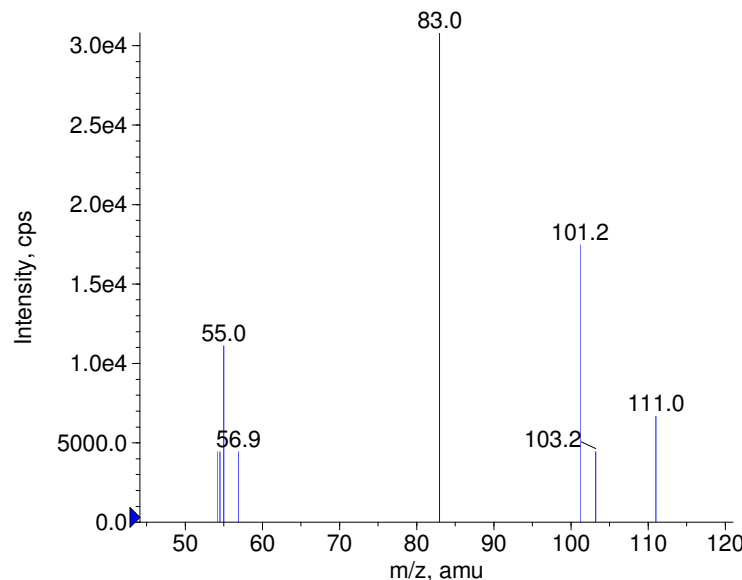
+ Dibutyl adipate Prec(259.0) CE(50.0) RT(3.7)
