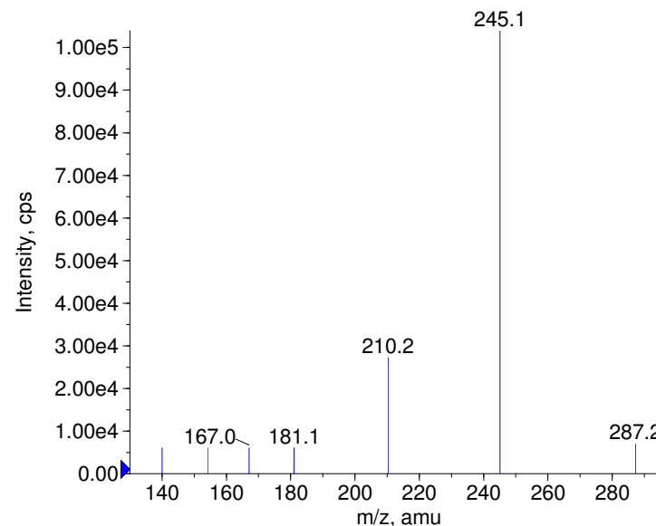
+ Desmethylobazam Prec(287.0) CE(99.0) RT(0.7)
