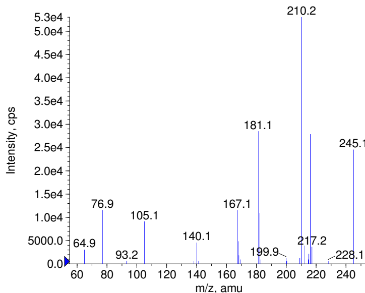
+ Desmethylobazam Prec(287.0) CE(50.0) RT(0.7)
