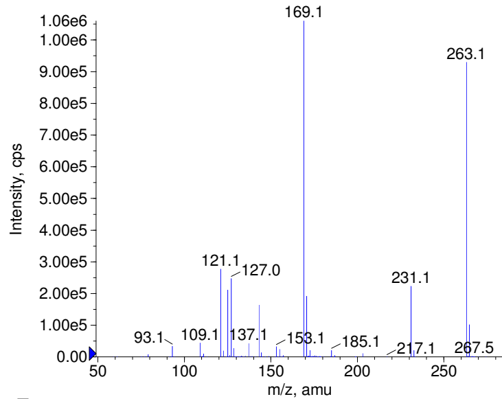
+ Demeton-S-methylsulfone Prec(263.0) CE(50.0) RT(0.9)
