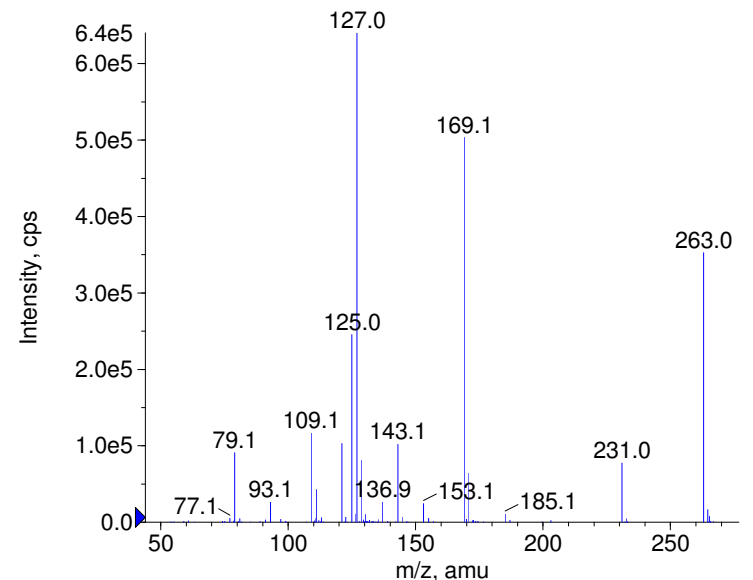
+ Demeton-S-methylsulfone Prec(263.0) CE(99.0) RT(0.9)
