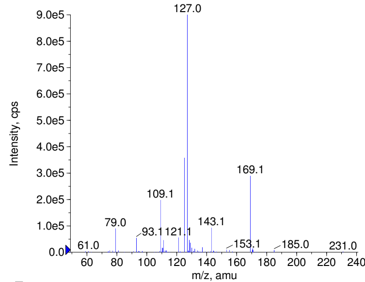
+ Demeton-S-methylsulfone Prec(263.0) CE(99.0) RT(0.9)
