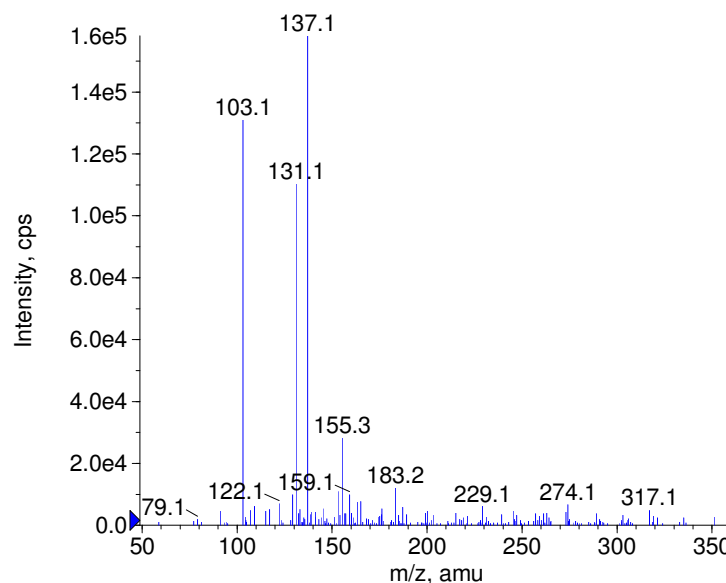
■ + Cyclovalone Prec(367.0) CE(50.0) RT(1.1)
