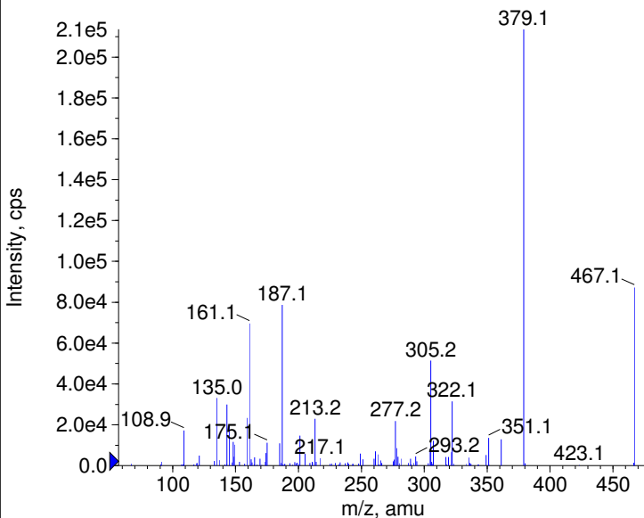
■ - Cromoglicic acid Prec(467.0) CE(-99.0) RT(0.9)
