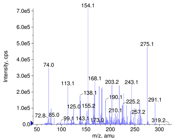
■ + Clotiazepam Prec(319.0) CE(50.0) RT(2.1)
