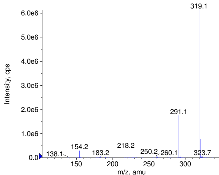
■ + Clotiazepam Prec(319.0) CE(50.0) RT(2.1)
