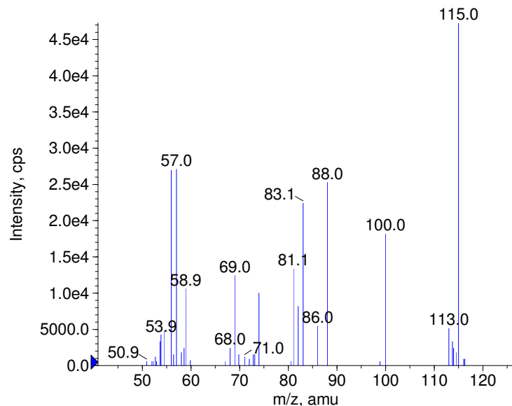
■ + Carbimazole Prec(187.0) CE(50.0) RT(0.8)
