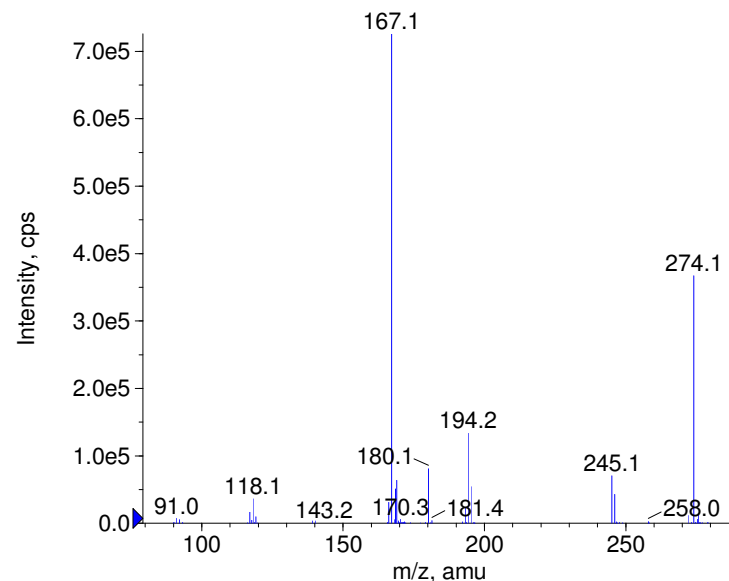
+ Brompheniramine Prec(319.0) CE(50.0) RT(0.7)
