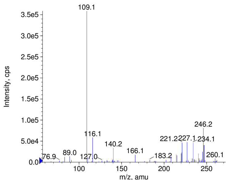
■ + Bidesmethylcitalopram Prec(297.0) CE(50.0) RT(12.1)
