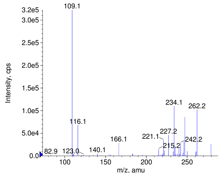
■ + Bidesmethylcitalopram Prec(297.0) CE(99.0) RT(12.2)
