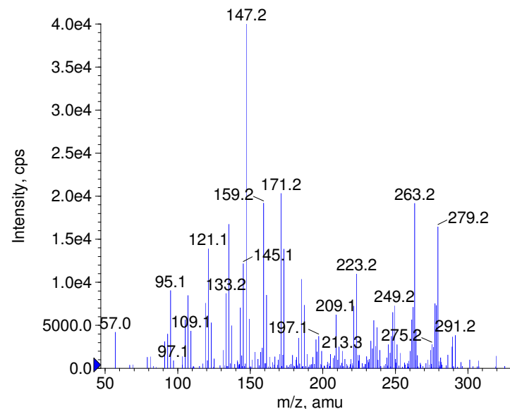
+ Betamethasone-17-valerate Prec(477.0) CE(50.0) RT(2.4)
