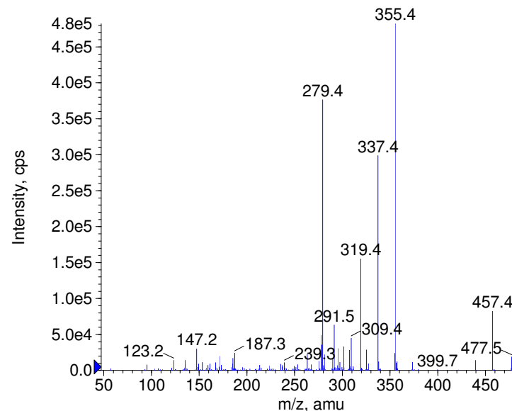
+ Betamethasone-17-valerate Prec(477.0) CE(50.0) RT(2.4)
