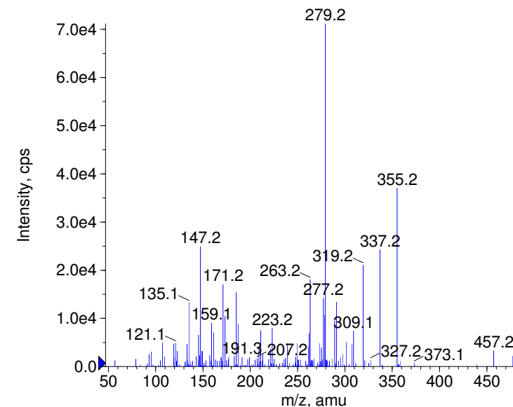
+ Betamethasone-17-valerate Prec(477.0) CE(99.0) RT(2.4)
