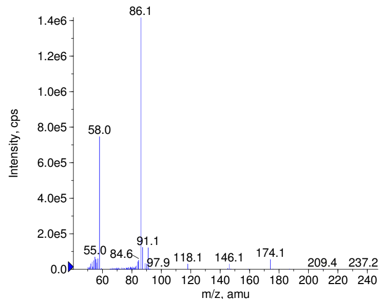
+ Benzydamine Prec(310.0) CE(50.0) RT(0.9)
