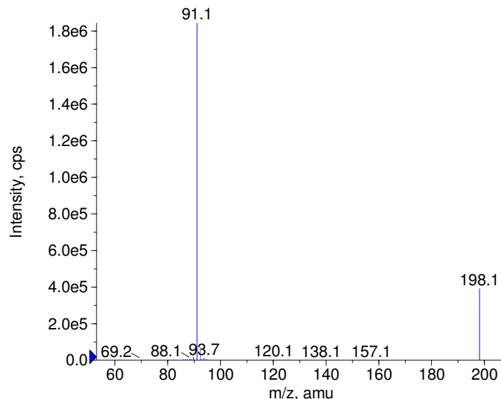
+ Beclamide Prec(198.0) CE(50.0) RT(1.2)
