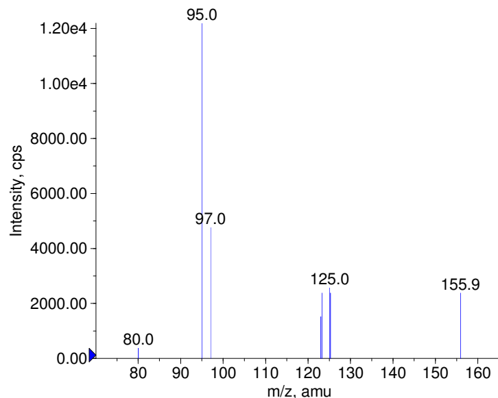
■ - Azelaic Acid Prec(187.0) CE(-50.0) RT(0.9)
