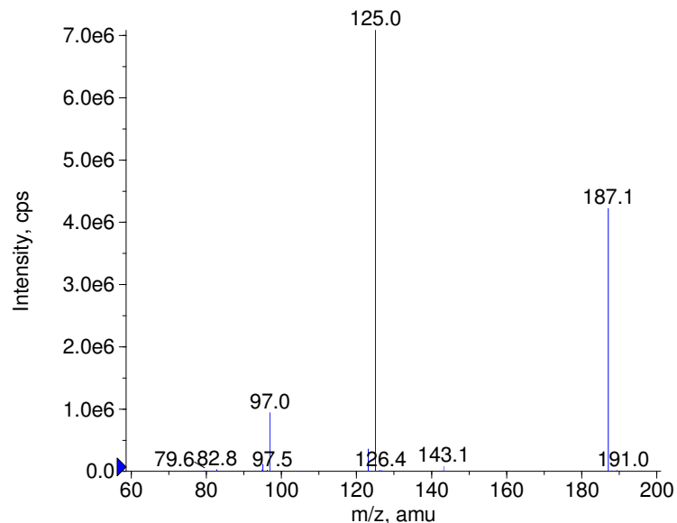
■ - Azelaic Acid Prec(187.0) CE(-50.0) RT(0.9)
