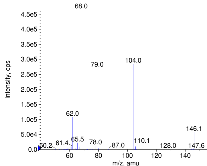
+ Atrazine-desethyl Prec(188.0) CE(50.0) RT(1.0)
