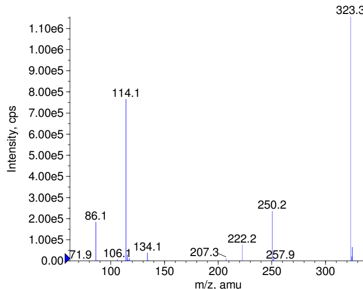
+ Aprinidine Prec(323.0) CE(50.0) RT(0.8)
