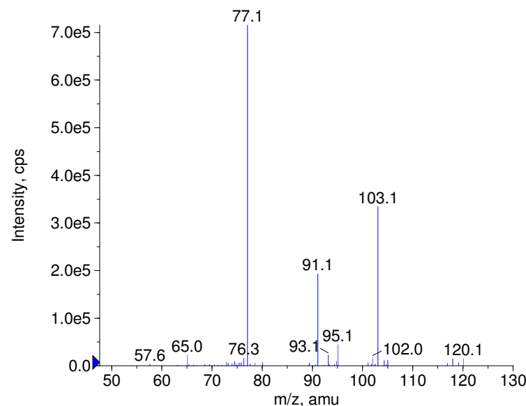
+ Aminorex Prec(163.0) CE(50.0) RT(0.9)
