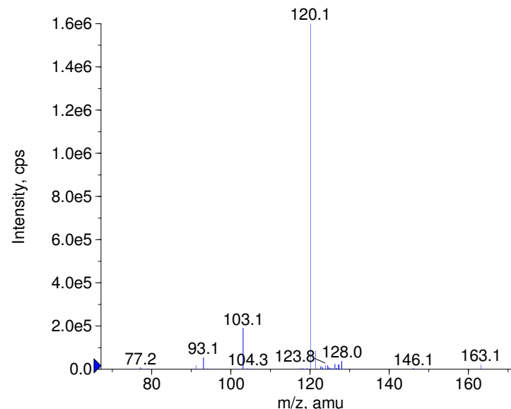
+ Aminorex Prec(163.0) CE(50.0) RT(0.9)
