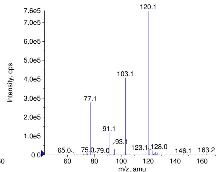
+ Aminorex Prec(163.0) CE(99.0) RT(0.9)
