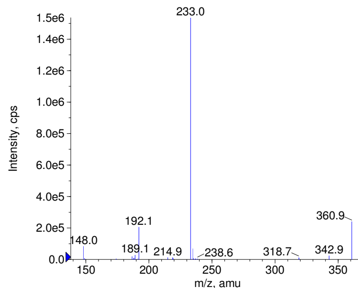
+ Amidotrizoic Acid Prec(615.0) CE(50.0) RT(0.9)
